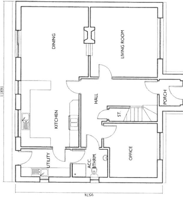
GROUND FLOOR PLAN AS PROPOSED 1/100
