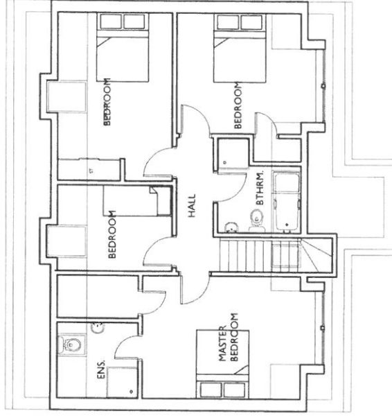
UPPER FLOOR PLAN AS PROPOSED 1/100
